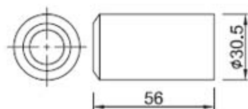
SLEEVES
