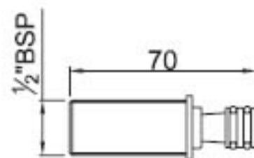
SPOUT NIPPLE
