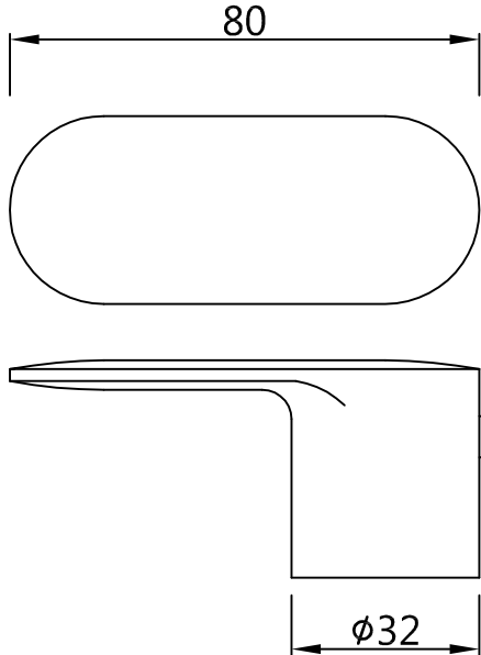
HANDLE
