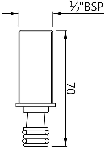
SPOUT NIPPLE
